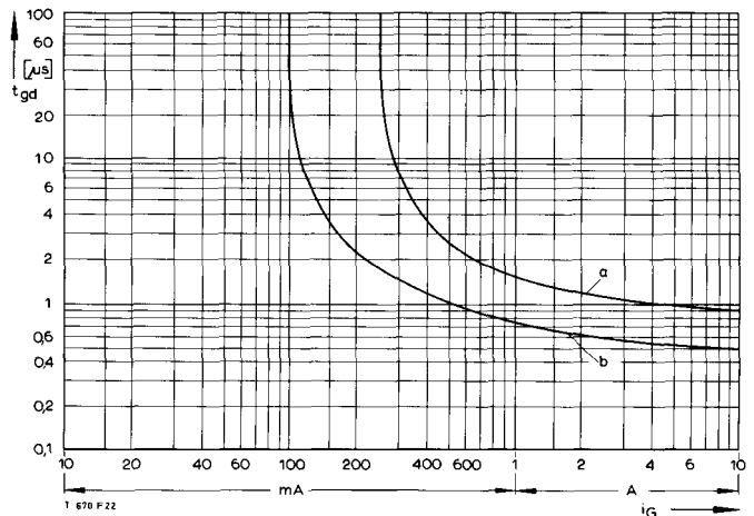
BildFig. 16 Zündverzugs/Gate controlled delay time t_{gd} = f(I_{GM}) , t_{vj} = 25^\circ C , di_G/dt = i_{GM}/1 ps a – Maximaler Verlauf/Limiting Characteristic b – Typischer Verlauf/Typical Characteristic
